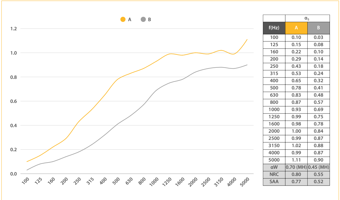
This graph shows the sound absorption coefficient of two pieces of Melamine Foam, tested separately and placed directly on the floor: • A: 40 mm thick • B: 20 mm thick
