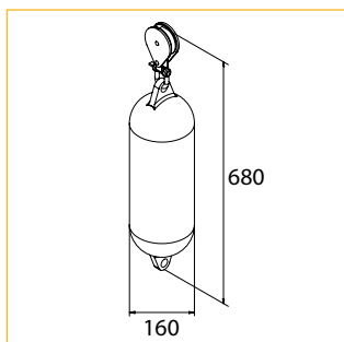
24. Weighted Return Pulley XL
