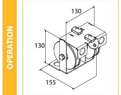
19. Head Pulley
