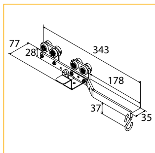
17. Overlap Carrier Set for Motor Control
