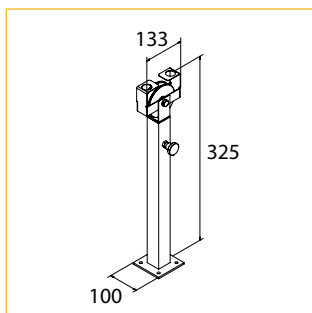
25. Floor Fixed Return Pulley
