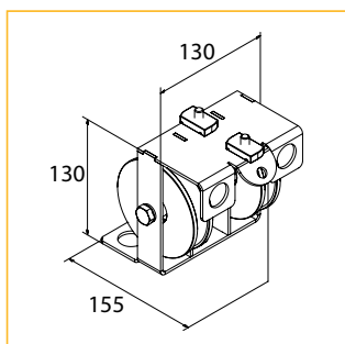
20. Head Pulley
