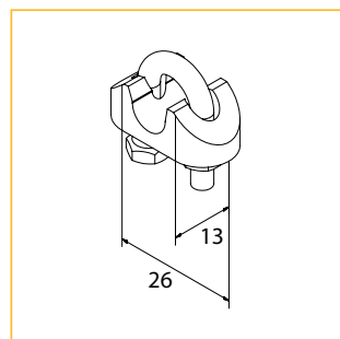
19. Rope Clamp (set of 3)
