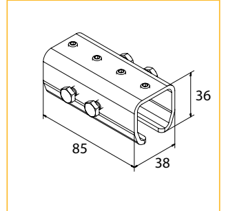
5. Coupling for use with Ceiling Brackets
