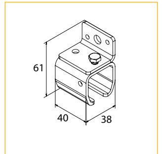
8. Wall Bracket
