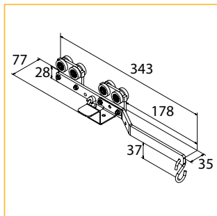
20. Overlap Carrier Set for Motor Control
