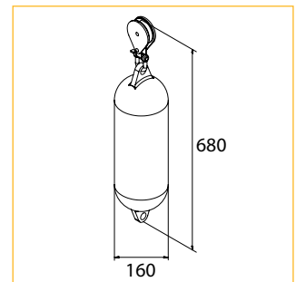
26. Weighted Return Pulley XL
