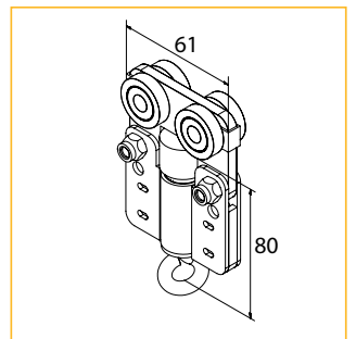
15. Master Carrier with Brake
