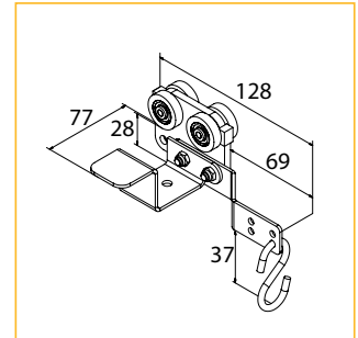
19. Short Overlap Carrier for Motor Control
