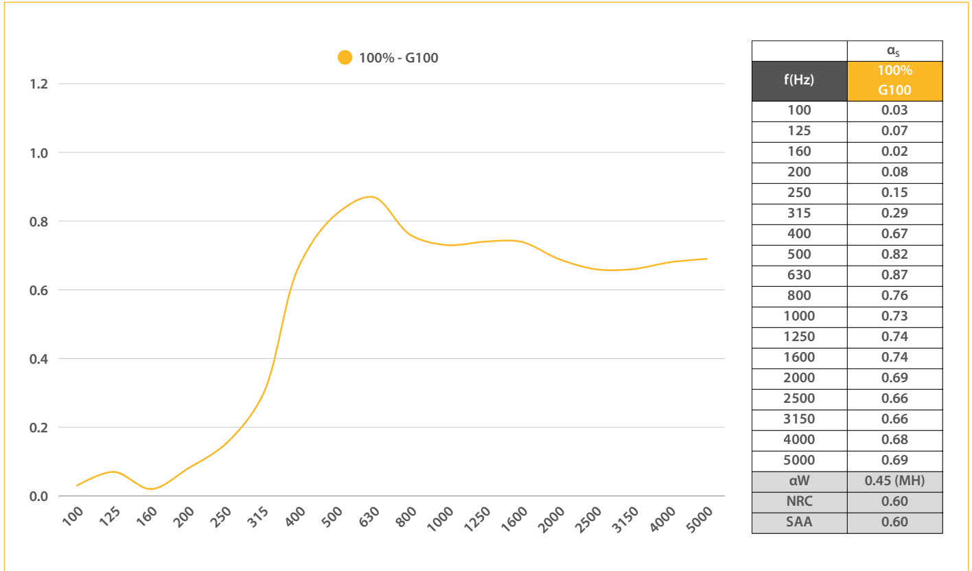
This graph shows the sound absorption coefficient of a 100% pleated curtain hung from a rail positioned 10 cm from the wall (G100).
