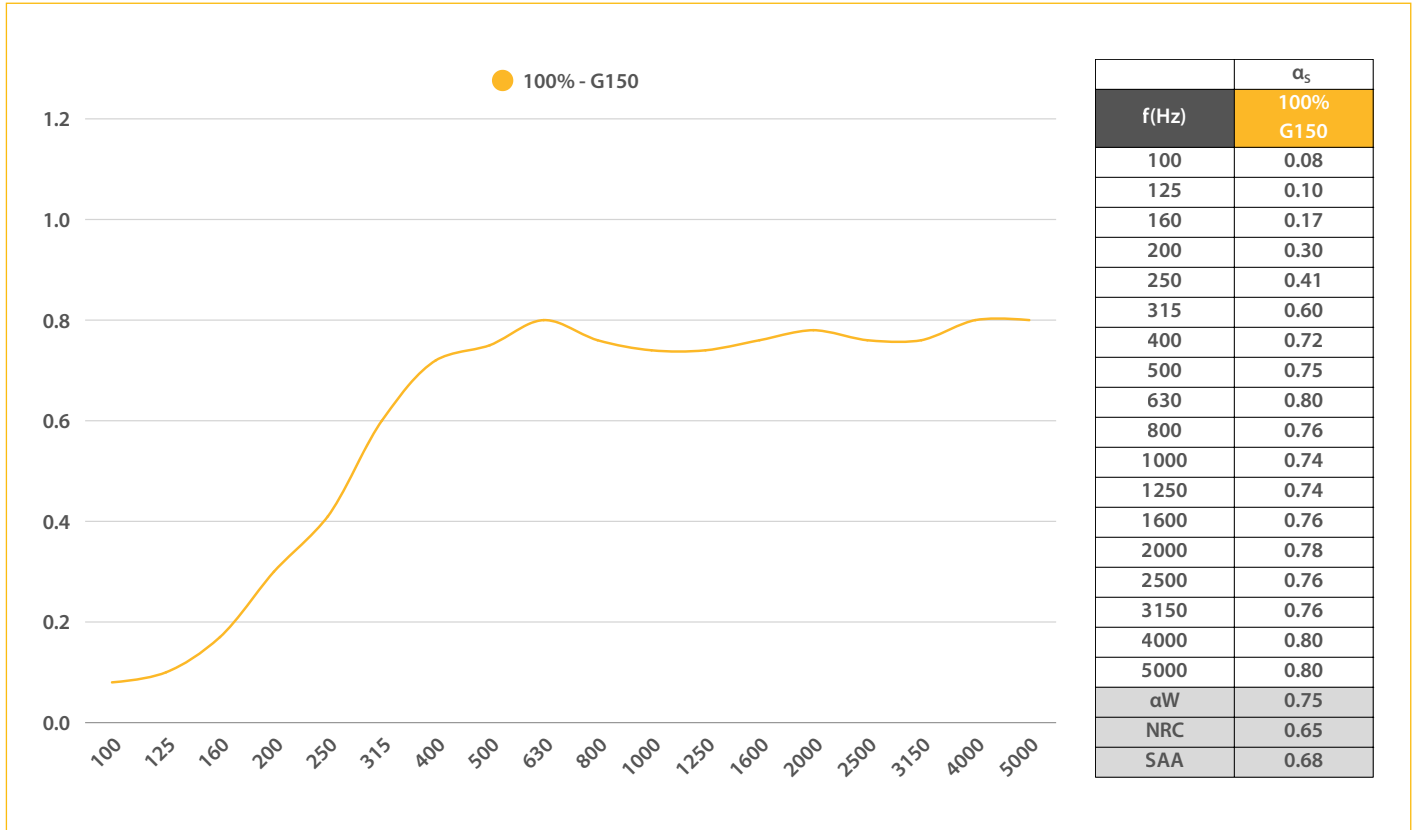
This graph shows the sound absorption coefficient of a 100% pleated curtain hung from a rail positioned 15 cm from the wall (G150).
